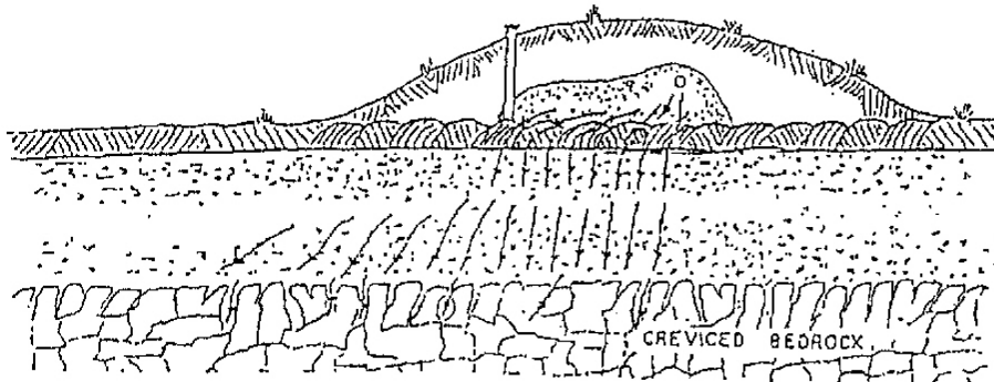
Figure 2: Linear Loading Rates for an At-Grade System.
