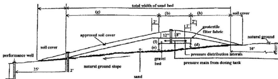
Figure 5: Plan and profile view of Mound System
